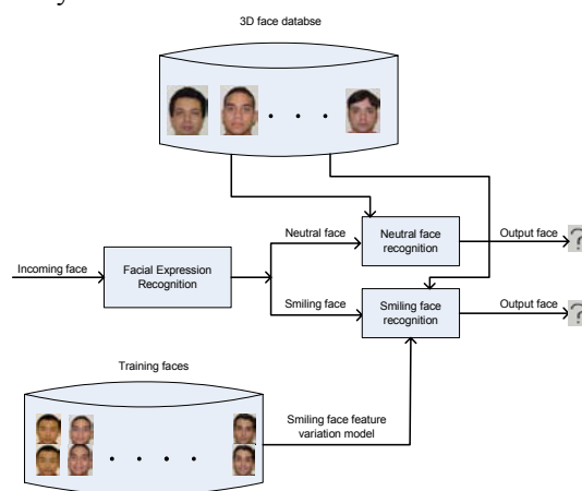
Figure1 Simplified framework of 3D face recognition
